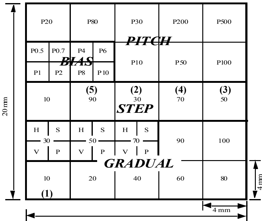
SKW 7-2 Mask Floor Plan
