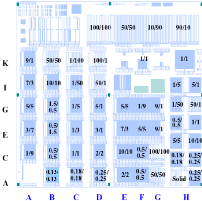
6-3TEOS(0.13) Mask Floor Plan
