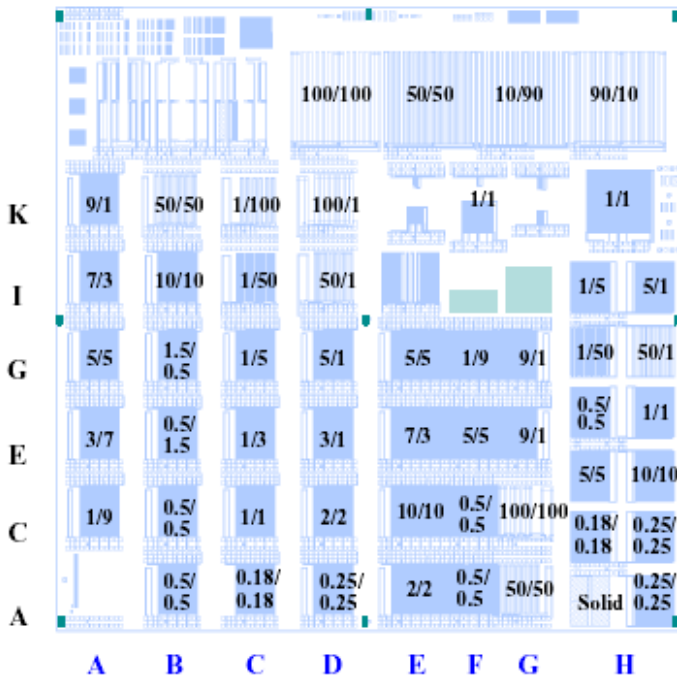
6-3TEOS(0.18) Mask Floor Plan
