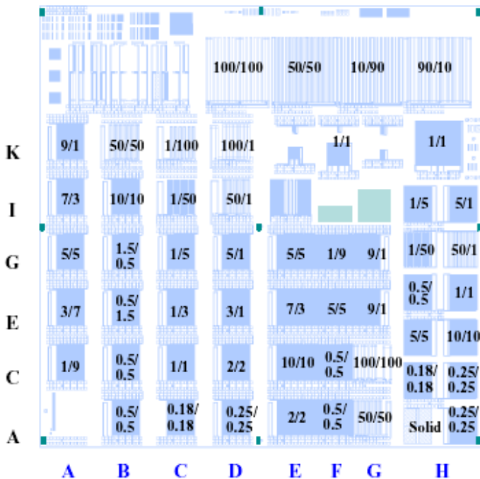
SKW6-3 (Cu/Coral) Mask Floor Plan
